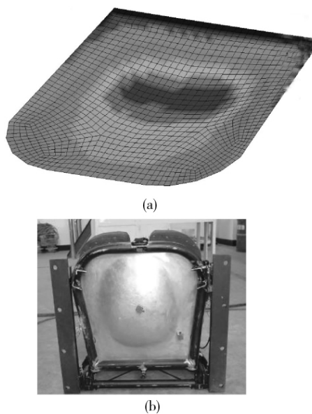
Fig. 8 Seat pan deformation
