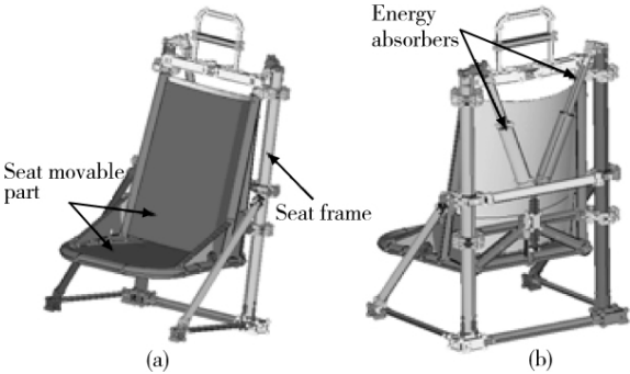
Fig. 2 Helicopter seat structure
