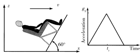
Fig. 1 Dynamic test requirement
